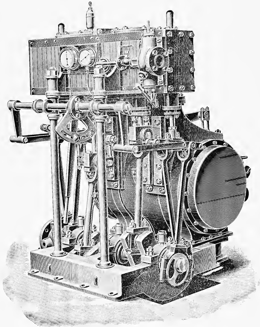
THE HAYES COMPOUND MARINE ENGINE.
